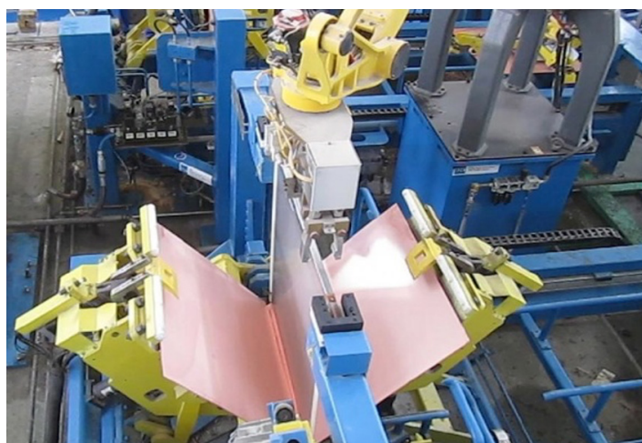
ROBOTIC-TYPE CSM
